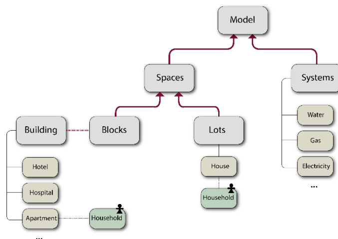
Figure 1. Model Entities.
