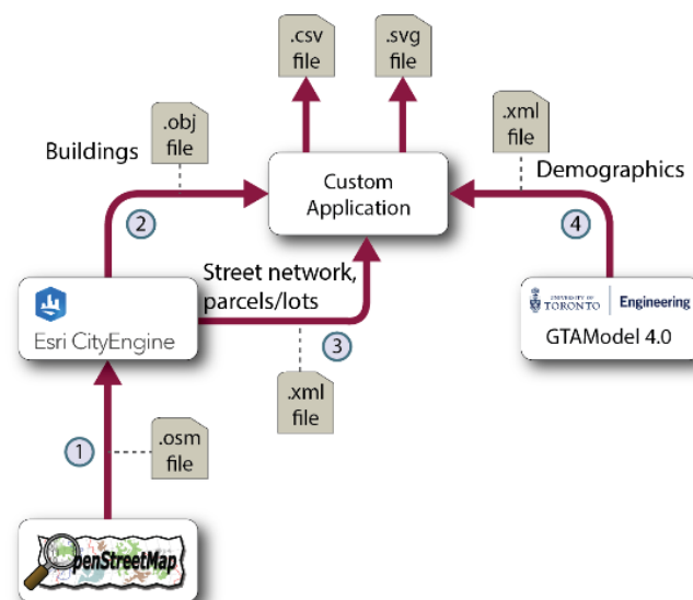
Figure 6. Dataflow.
