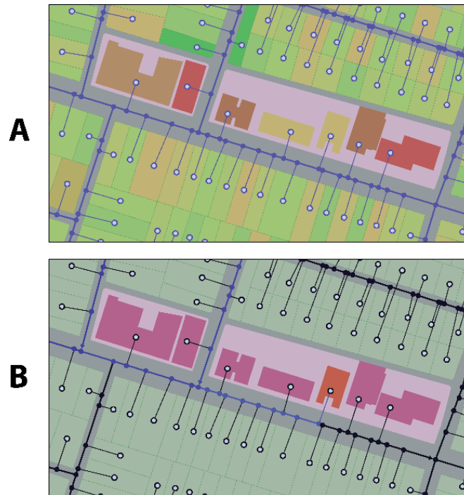
Figure 12. Interactive Visualizations.
