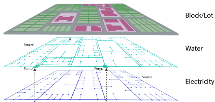
Figure 10. Dependencies between subsystems.
