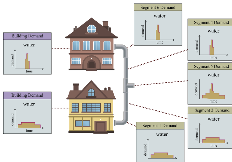
Figure 4. Demand propagation.
